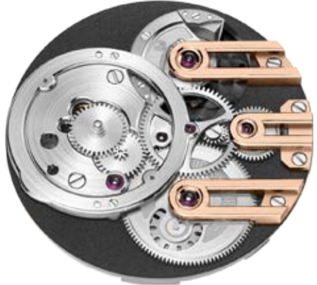
A look at the watch's mechanism
